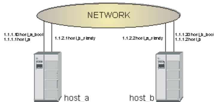
Figure 4. Sample environment for HACMP takeover
